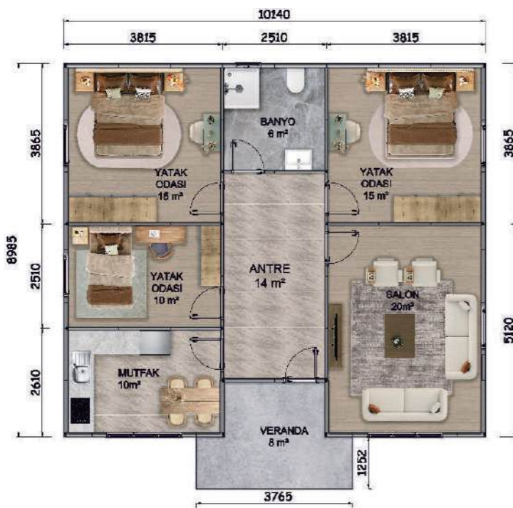
Tek Katlı Prefabrik Konut Single Storey Prefabricated House 90m 2 + 8m 2 Veranda
